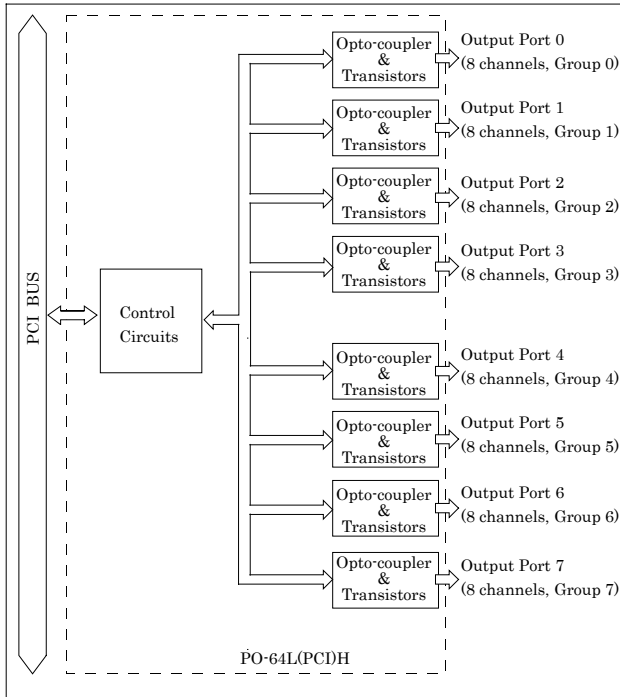
Figure 6.3. Block Diagram < PO-64L(PCI)H >
