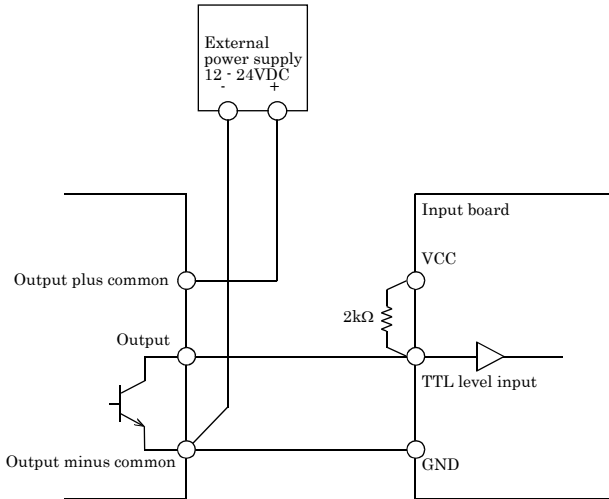
Figure 3.15. Connection Example of Output and TTL level Input Signal <PIO-32/32L(PCI)H>, <PO-64L(PCI)H>
