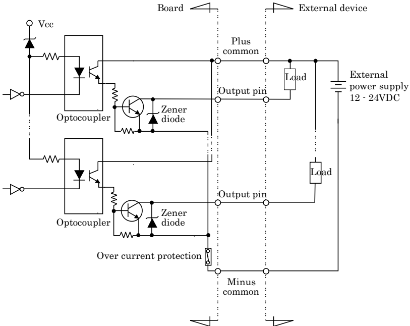
Figure 3.13. Output Circuit <PIO-32/32L(PCI)H>, <PO-64L(PCI)H>
