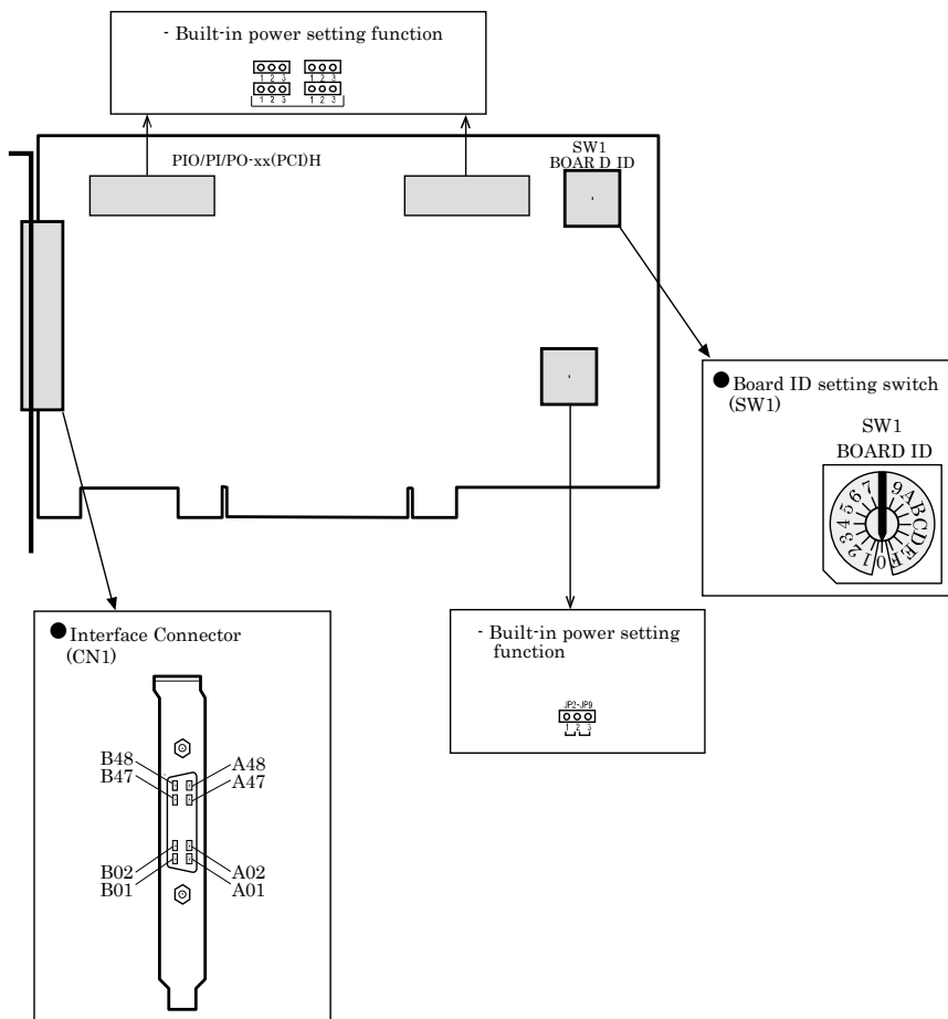
Figure 2.1. Component Locations
