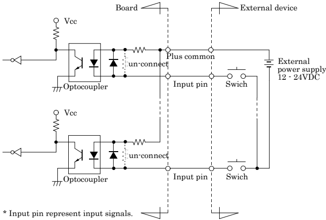
Figure 3.11. Input Circuit <PIO-32/32L(PCI)H>, <PI-64L(PCI)H>
