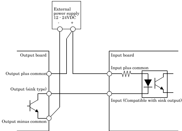
Figure 3.16. Example of Connecting the Sink Type Output and Sink Output Support Input
