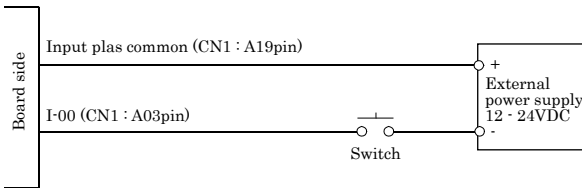
Figure 3.12. An Example to use Input I00 <PIO-32/32L(PCI)H>, <PI-64L(PCI)H>
