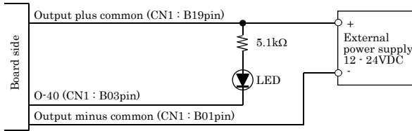
Figure 3.14. An Example to use Output O-40 <PIO-32/32L(PCI)H>, <PO-64L(PCI)H>
