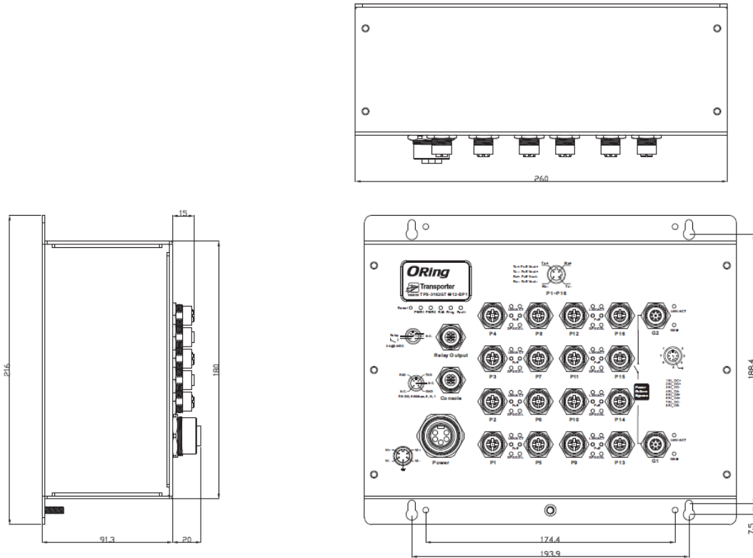
Wall-mount Measurement
